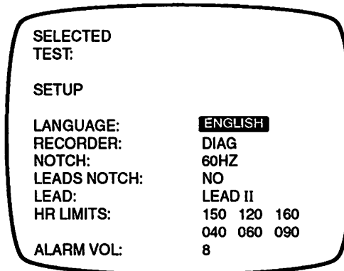
Figure 3-3 Setup Menu
