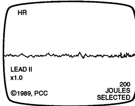
Figure 3-1 Power-On Display
