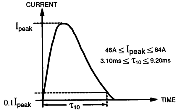
Figure 3-10 Output Waveform
