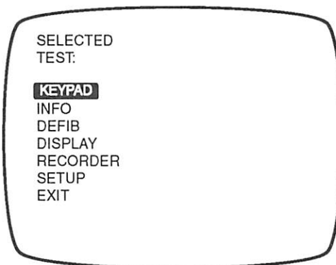
Figure 2-3 Test Menu
