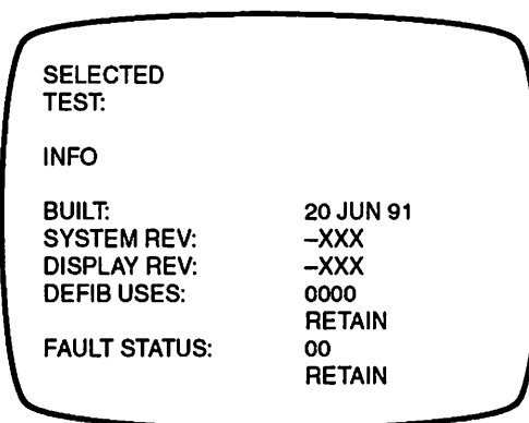
Figure 2-5 Info Menu
