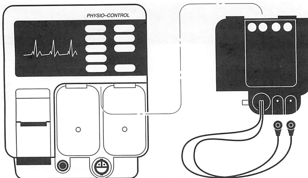
Figure 1-1 LIFEPAK 9 shock advisory adapter Location
