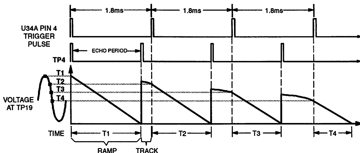
Figure 1-6 Echo Period
