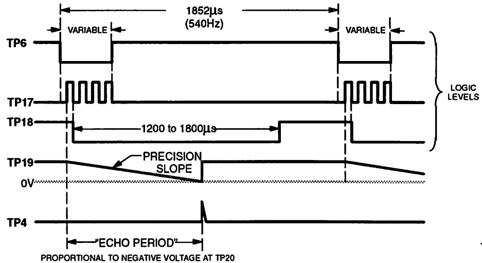
Figure 1-5 Preamp Timing
