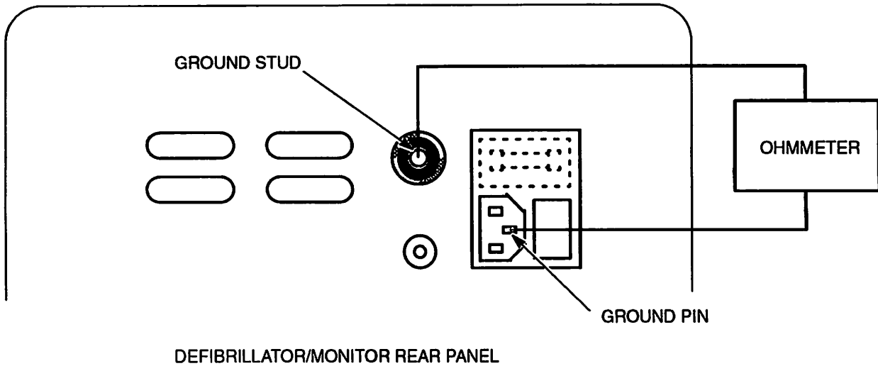
Figure 3-7 Test Connections for Ground Resistance Measurement
