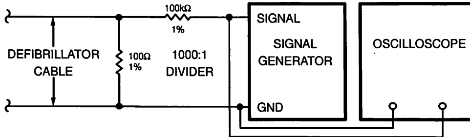
Figure 3-2 Test Signal Setup
