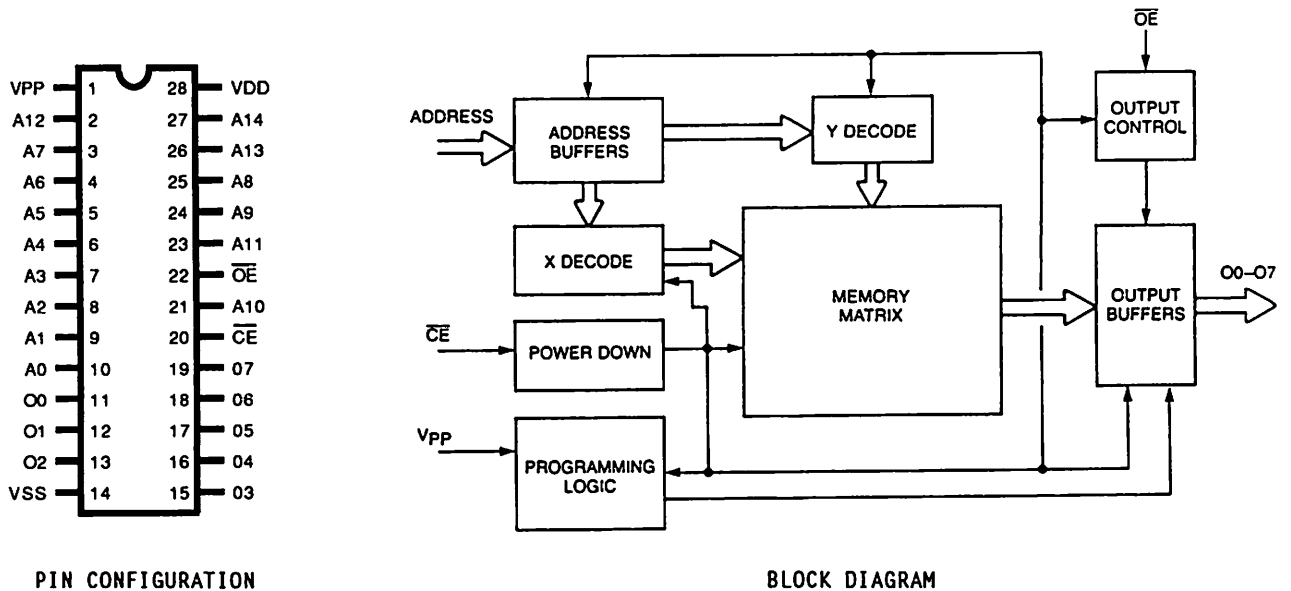
Figure 6-10 EPROM
