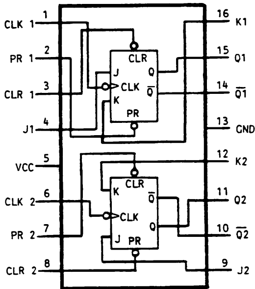
CONNECTION DIAGRAM
