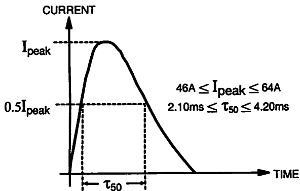
Figure 3 Output Waveform
