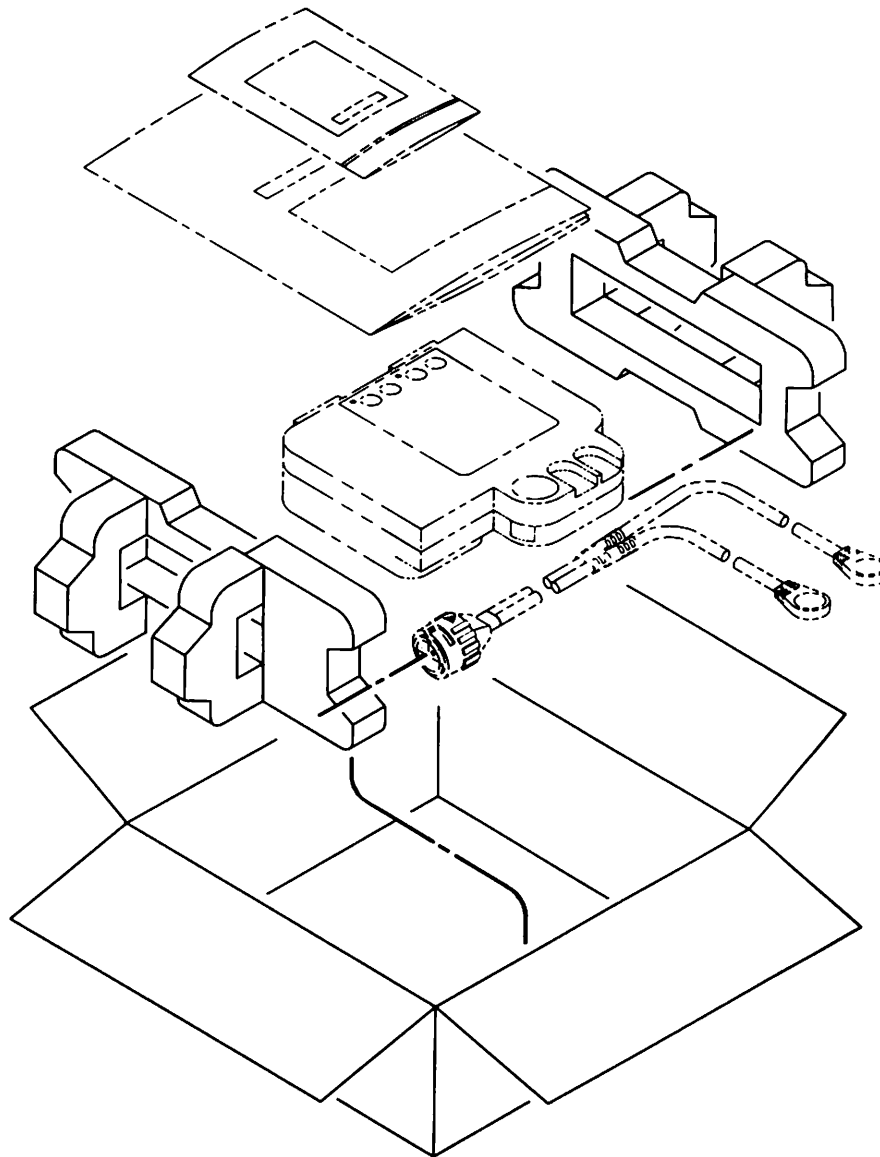
Figure 4-1 LIFEPAK 9 shock advisory adapter Shipping Assembly
