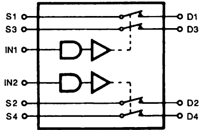
FUNCTIONAL DIAGRAM
