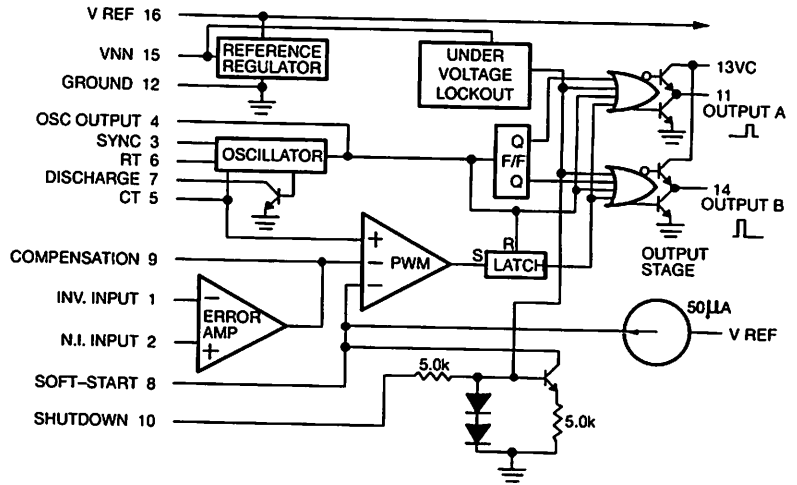
Figure 6-4 Pulse-Width Modulator
