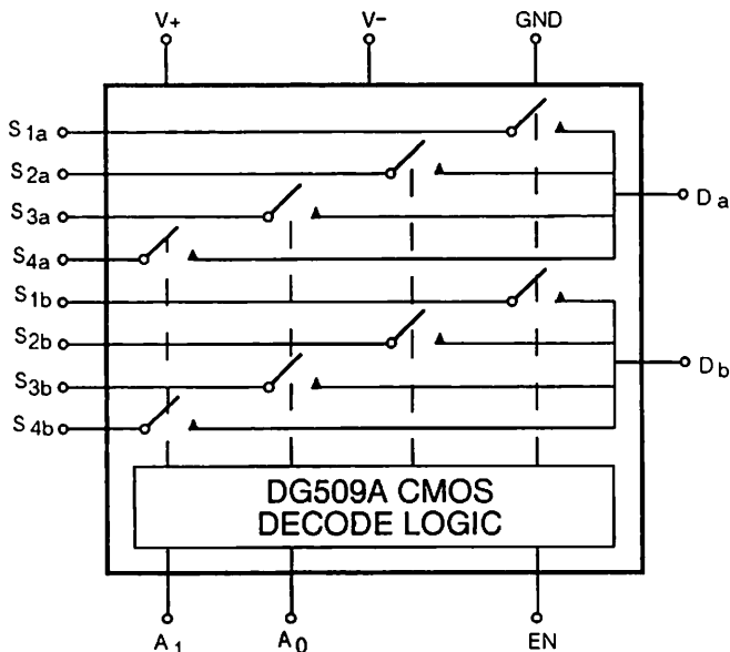
FUNCTIONAL DIAGRAM
