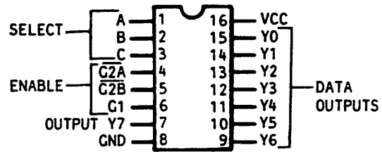
PIN CONFIGURATION
