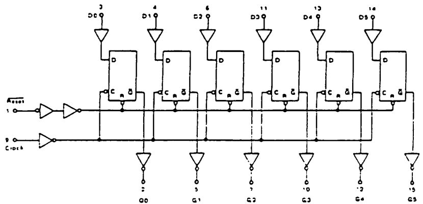
FUNCTIONAL DIAGRAM
