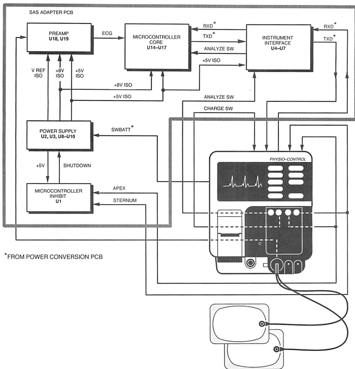
Figure 1-3 LIFEPAK 9 Shock advisory adapter Functional Block Diagram
