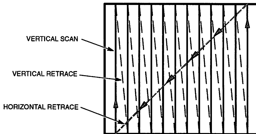
Figure 1-12 Display Scanning
