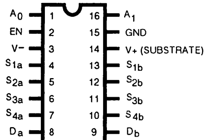
PIN CONFIGURATION
