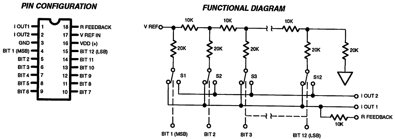
Figure 6-4 D/A Converter
