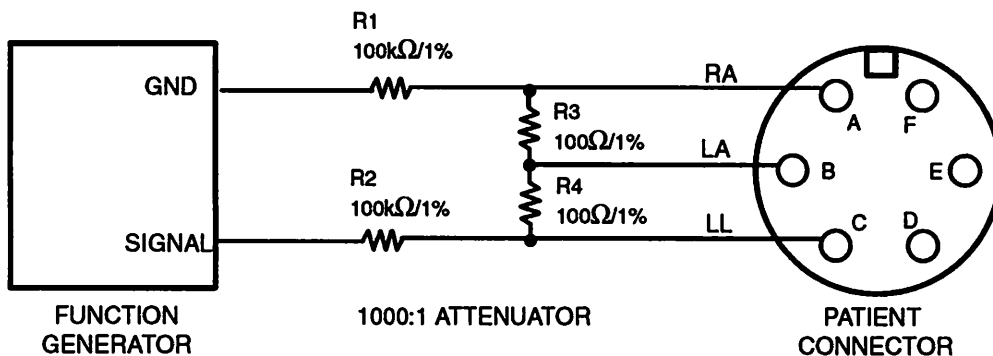
Figure 3–14 Test Signal Setup for Function Generator
