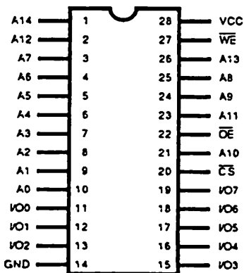
PIN CONFIGURATION
