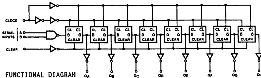
FUNCTIONAL DIAGRAM
