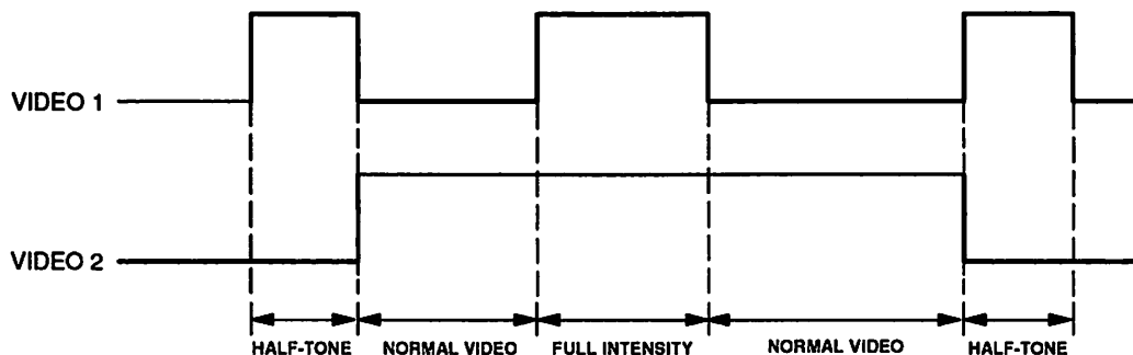
Figure 1-9 Video Intensity
