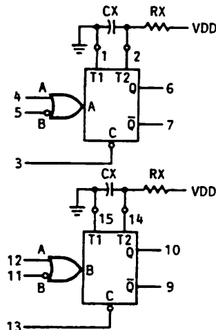
FUNCTIONAL DIAGRAM
