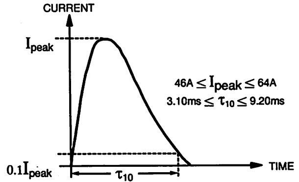
Figure 3 Output Waveform
