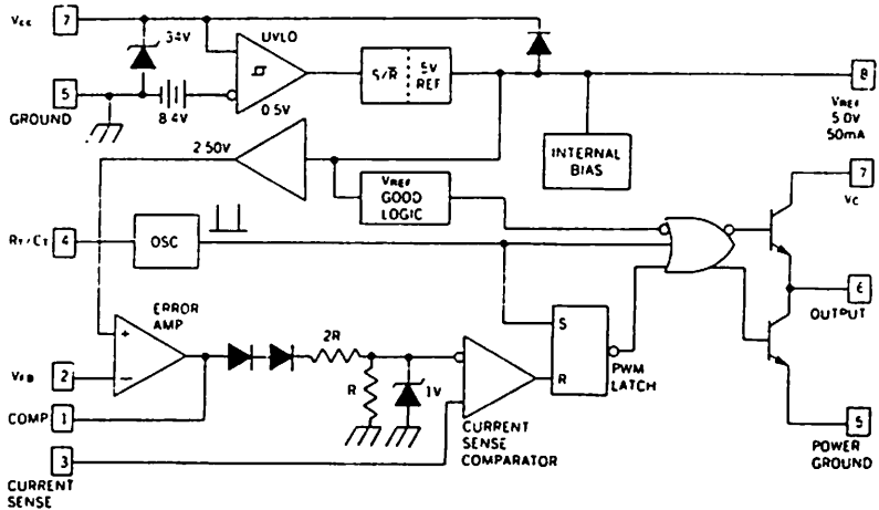
FUNCTIONAL DIAGRAM
