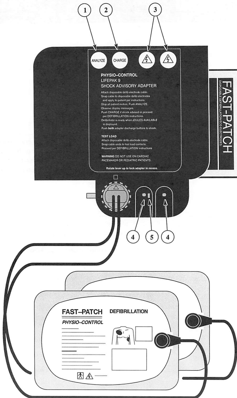
Figure 2-1 Front Panel Controls and Indicators
