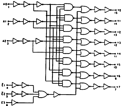
FUNCTIONAL DIAGRAM
