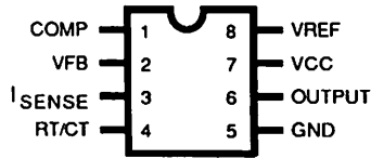
PIN CONFIGURATION
