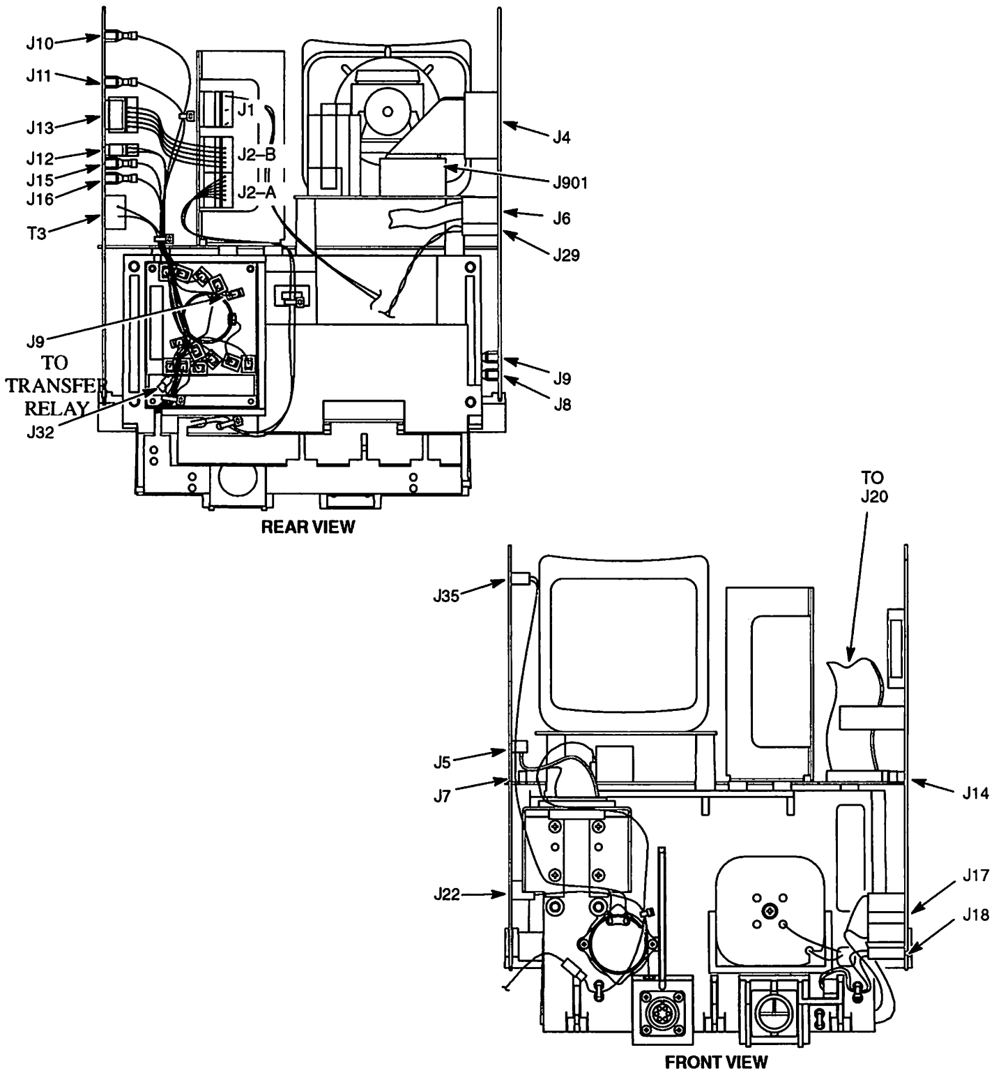
Figure 4-2 Connector Locations
