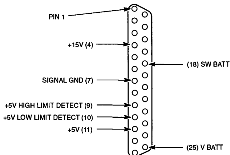
Figure 3–8 Test Connector J3
