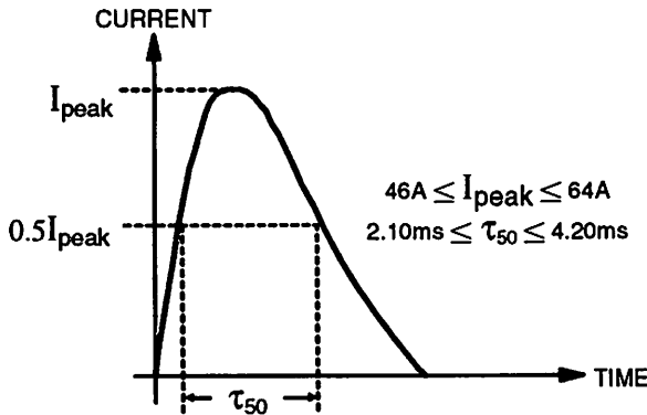
Figure 3-10 Output Waveform
