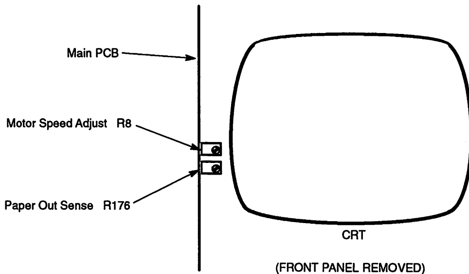
Figure 3-13 Recorder Calibration Adjustments Location
