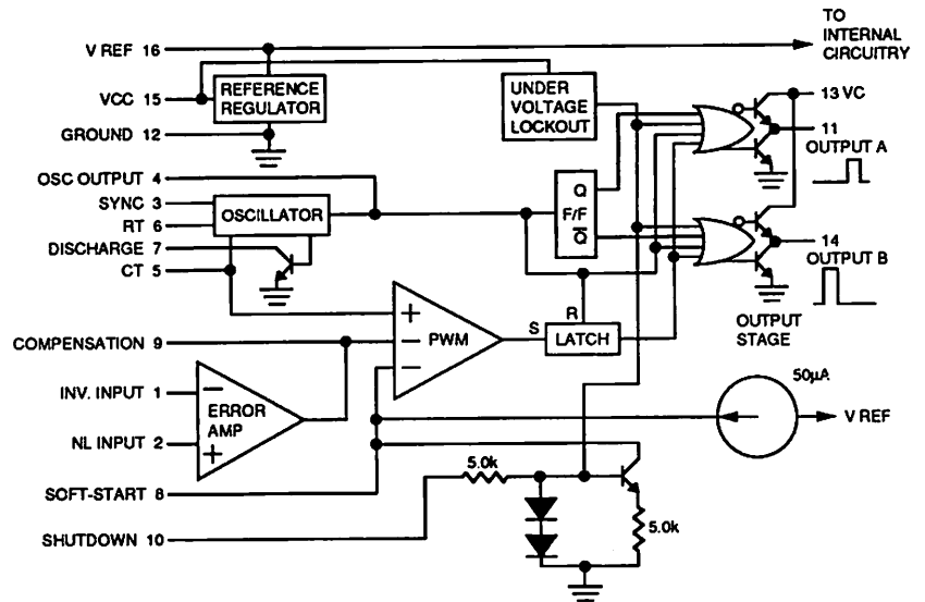
FUNCTIONAL DIAGRAM
