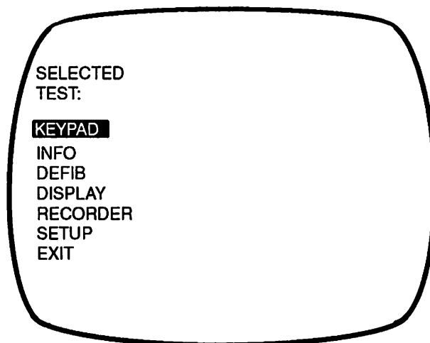
Figure 3–9 Test Menu
